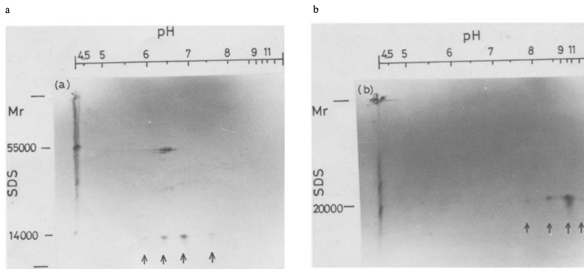
Fig.1. Two-dimensional gel electrophoresis of RuBPCase and of its precursor synthesized in vitro. (a) [ 35 S]Methionine-labeled RuBPCase was prepared and immunoprecipitated as in section 2. The immunoprecipitates were analyzed by isoelectric focusing and SDS-polyacrylamide gel electrophoresis, and fluorographed as described. (b) [ 35 S]Methionine-labeled precursor was prepared and immunoprecipitated as in [11]. The immunoprecipitates were treated as above.
